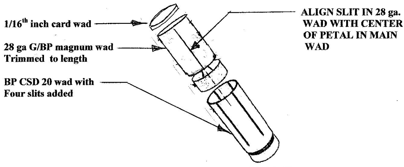
FIGURE A TUNGSTEN SUPER SHOT WAD COLUMN
